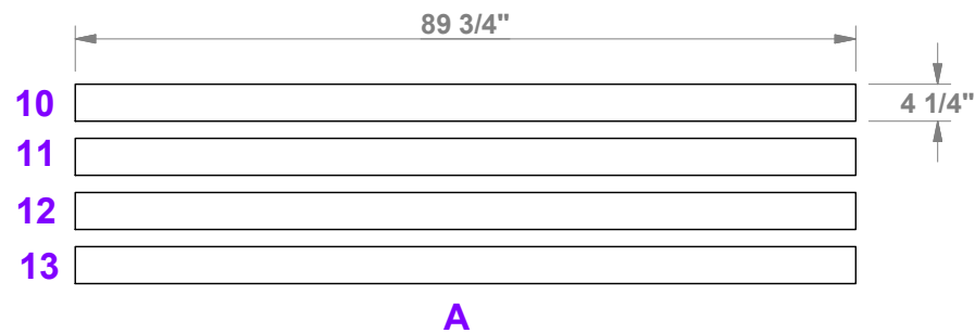
FLOOR PANELS - FLATTENED VIEW
